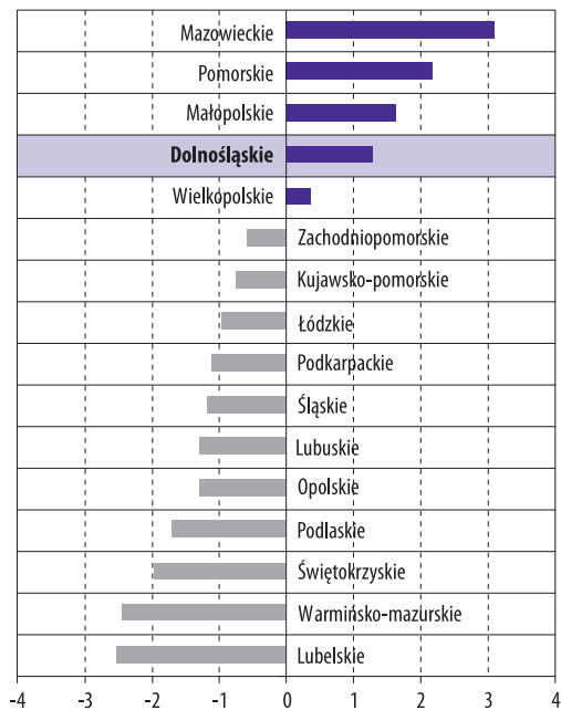
Chart 2. Internal and international net migration for permanent residence per 1000 population in 2018
